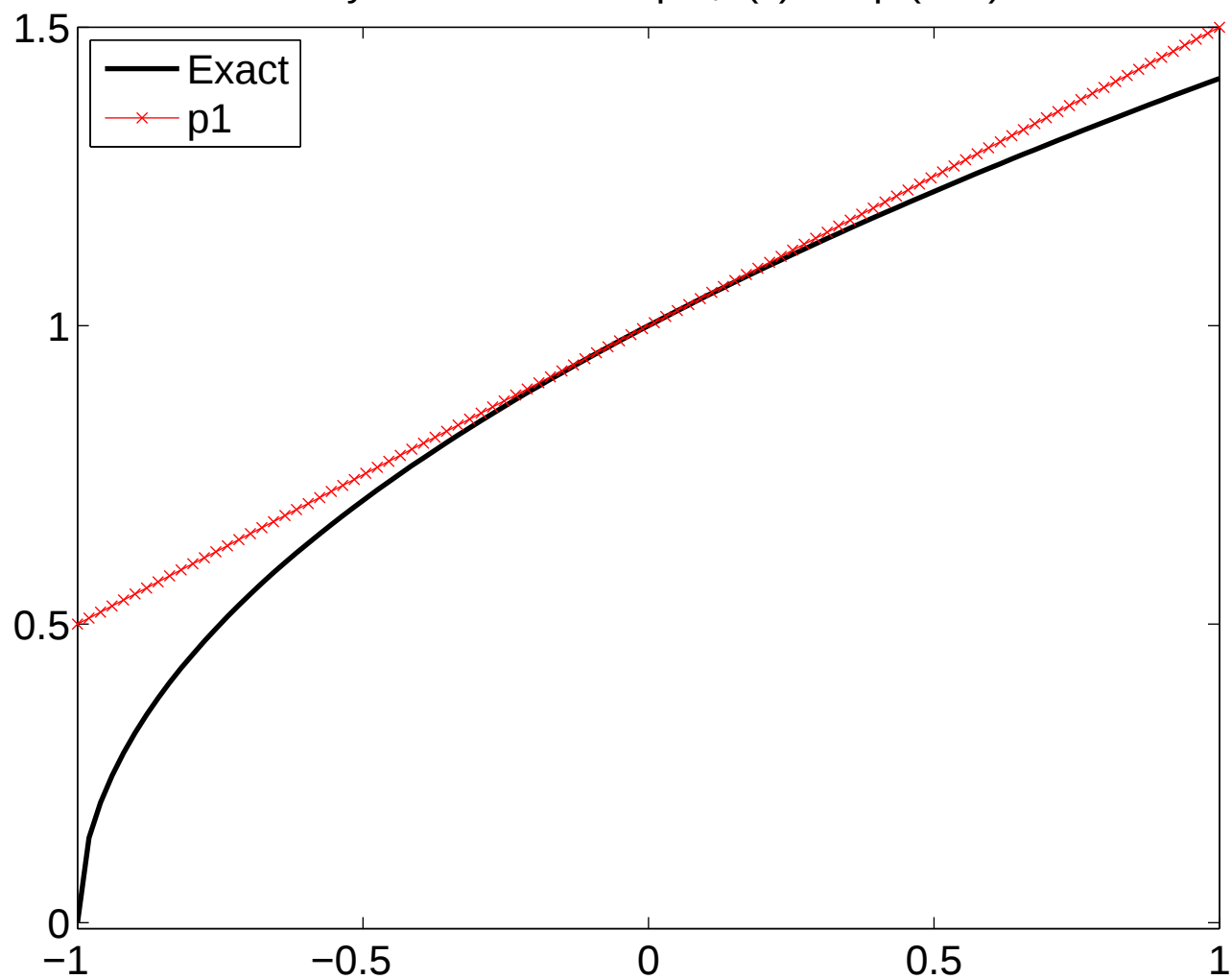
Taylor Series Example, f(x) = \sqrt{1+x}
