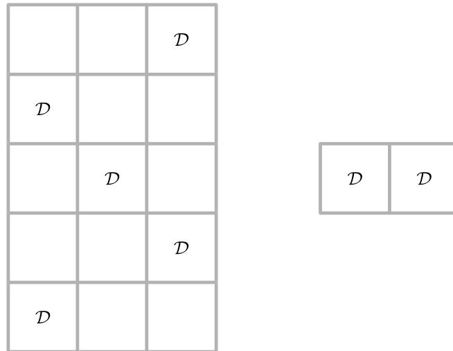
Fig. 7. The two types of permutation in Corollary 3.2.
