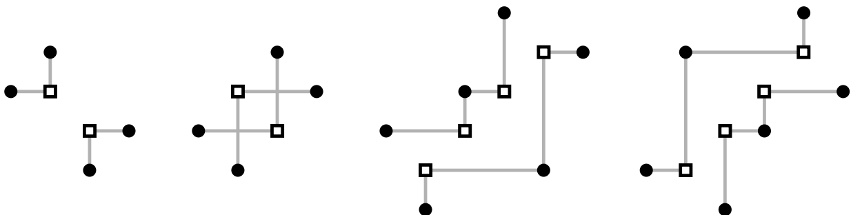
Fig. 9. Four illegal configurations for a permutation in Av(2341, 4123, 3412).
