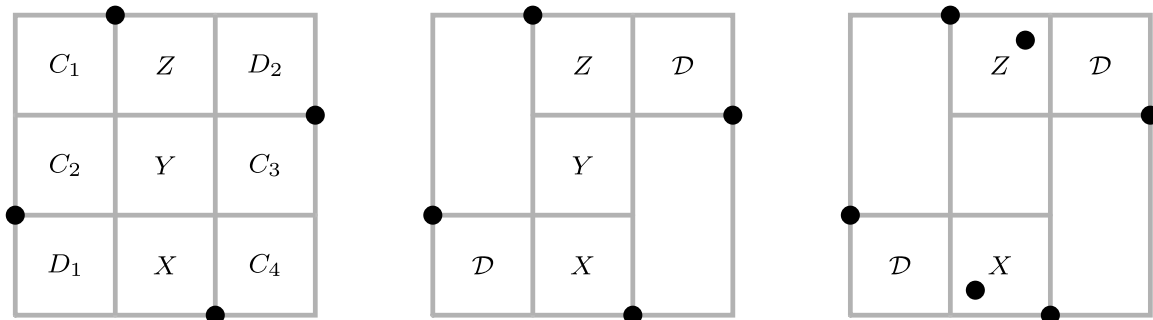
Fig. 6. Structure diagrams for a permutation in \text{Av}(2341, 4123, 3412) in which n precedes 1 but n is not the first entry and 1 is not the last entry.
