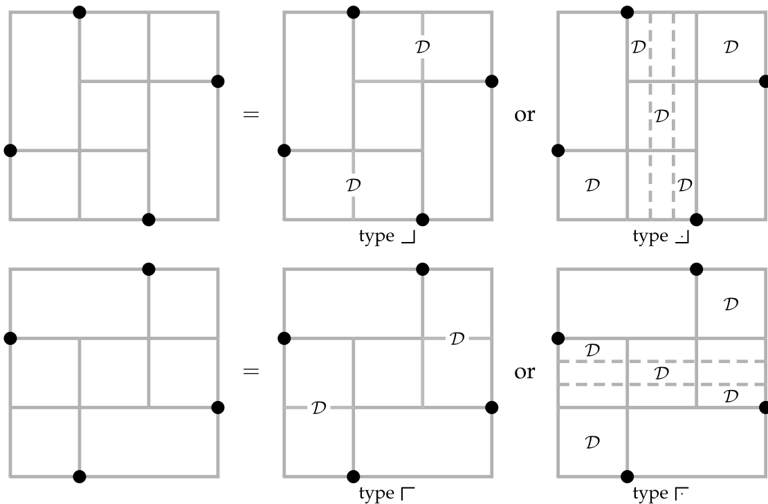
Fig. 11. The possible forms of the rectangles defined by two consecutive l–r maxes and two consecutive l–l mins in a simple permutation in Av(2341, 4123, 3412).
