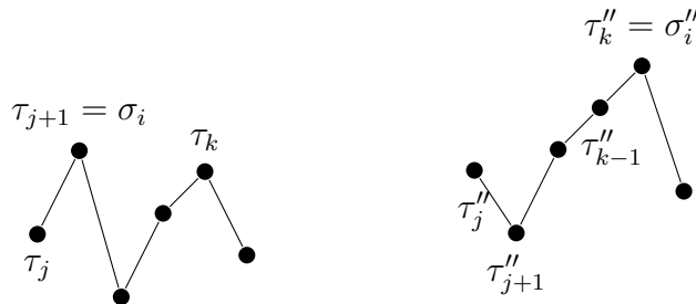
Figure 1: A schematic drawing for the case when 1 \leq x \leq \text{des}(\delta) + 1 and j + 2 \neq k .
