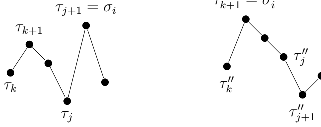
Figure 2: A schematic drawing for the case when \text{des}(\delta) + 2 \leq x \leq |\delta| + 1 modulo |\delta| + 1 .
