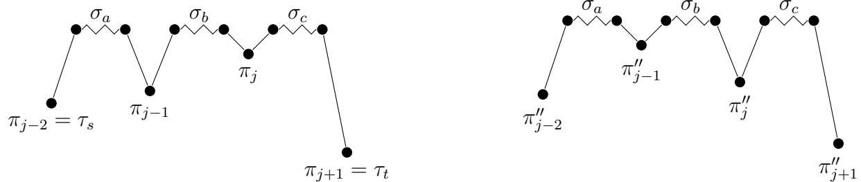
Figure 4: An illustration of the case when \sigma_a, \sigma_b, and \sigma_c are all nonempty.
