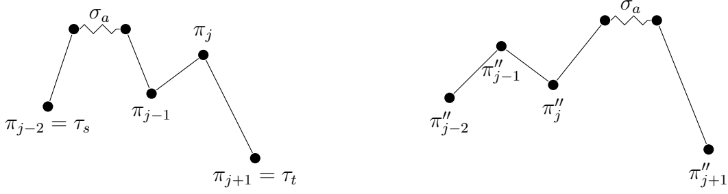
Figure 3: An illustration of the case when \sigma_a \neq \emptyset and \sigma_b = \sigma_c = \emptyset .
