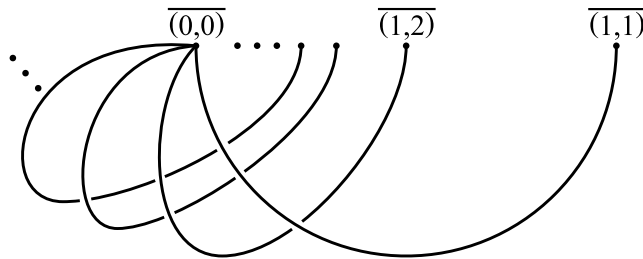
Fig. 3. Closed subspace A \subset HR .
