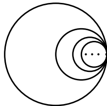
Fig. 4. Hawaiian earring HE \subset \mathbb{R}^2 .
