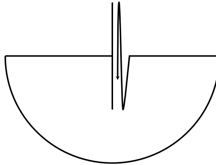
Fig. 1. Warsaw circle W \subset \mathbb{R}^2 .
