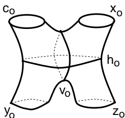
Fig. 10. “Horizontal” and “vertical” circles
