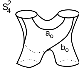
Fig. 6. Unlinked disjoint arcs of type 2
