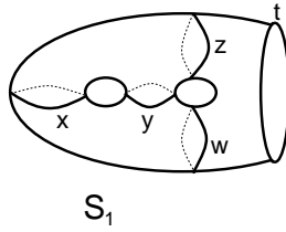
Fig. 4. Nonseparating circles, x, y, z , bounding a pair of pants
