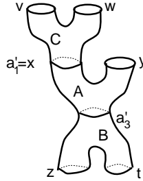
Fig. 3. Adjacent circles
