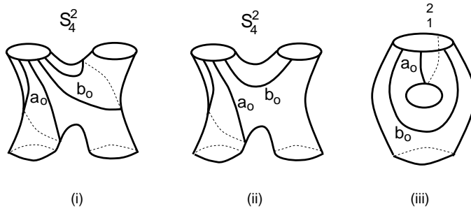
Fig. 9. Disjoint arcs and neighborhoods
