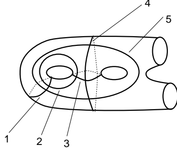
Fig. 5. Circles intersecting once
