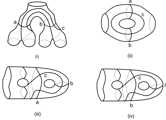
Fig. 1. Four possible cases for P_0
