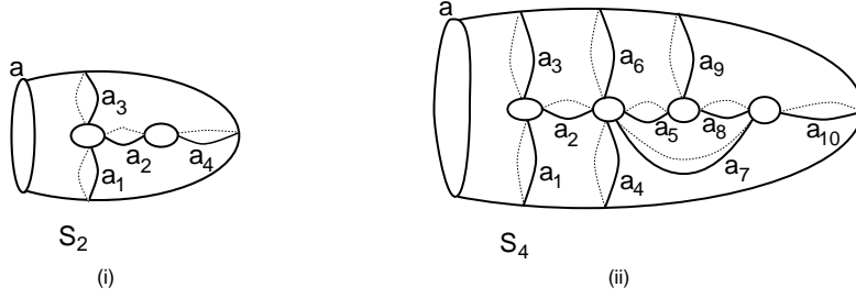
Fig. 2. Pants decompositions with separating circles
