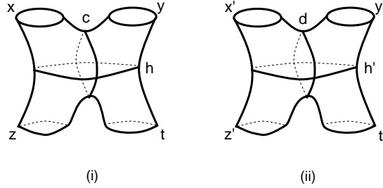
Fig. 14. Sphere with four holes
