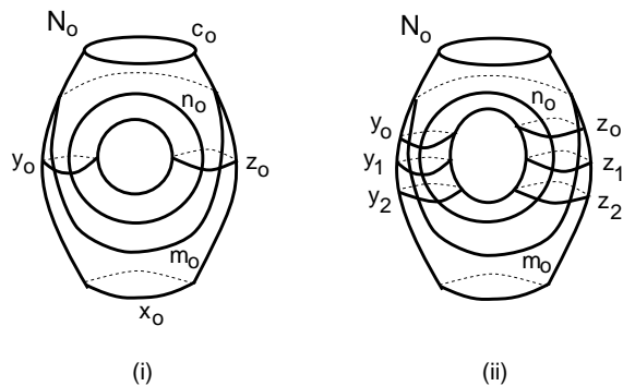
Fig. 12. Circles on torus with two boundary components
