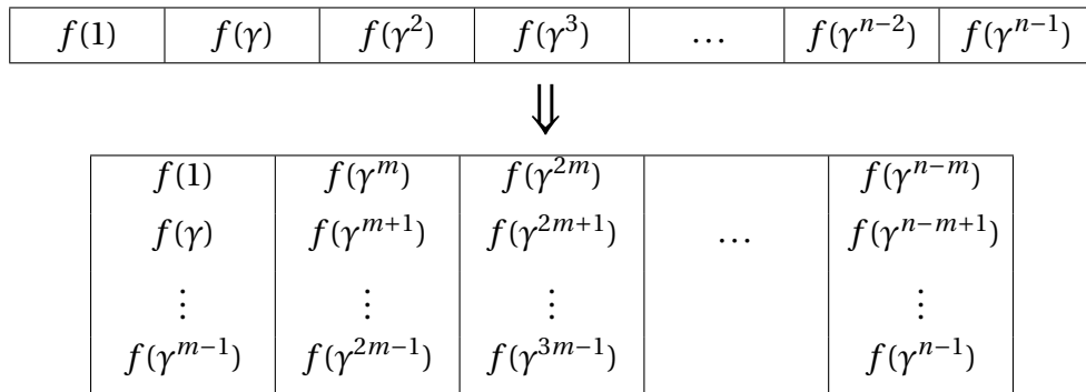
Figure 17.3: Folded Reed-Solomon code for general m \geq 1 .
