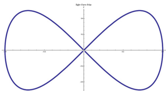
Figure 1: The Lemniscate
