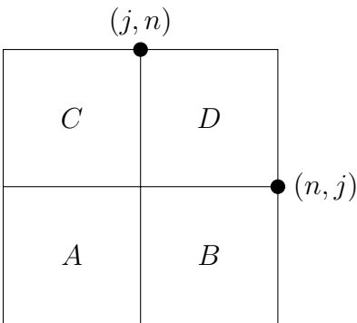
Figure 3: The diagram of \iota
