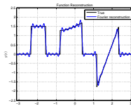
(c) Fourier reconstruction showing Gibbs
