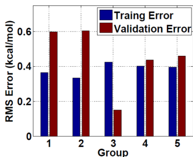
FIG. 10. The bar plot of the training and validation errors of the ethers.
